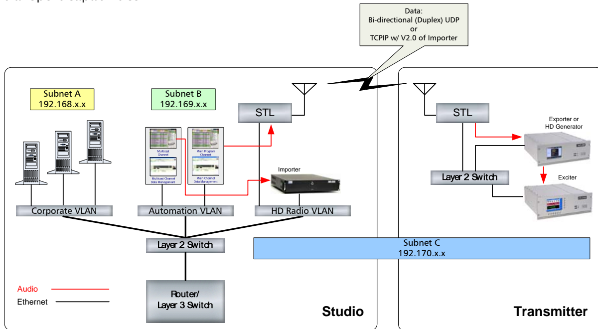
– Fig. 5: Multicast Network Architecture, HD Generation at Transmitter Site –
