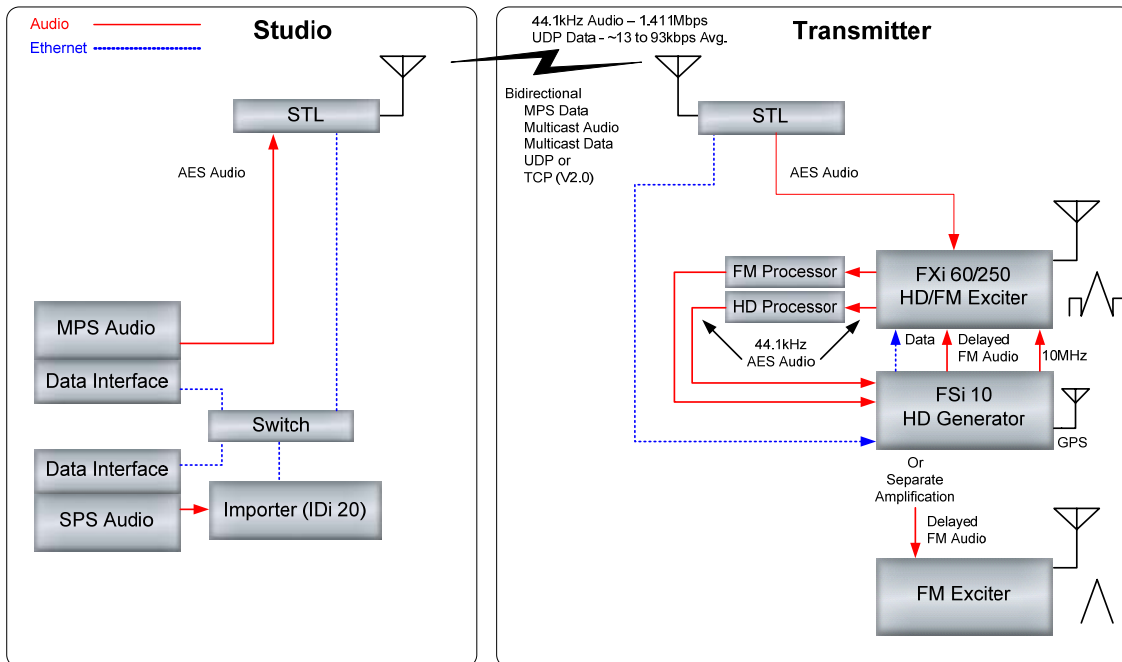
– Fig. 2: Multicast Architecture, HD Generation at Transmitter Site –
