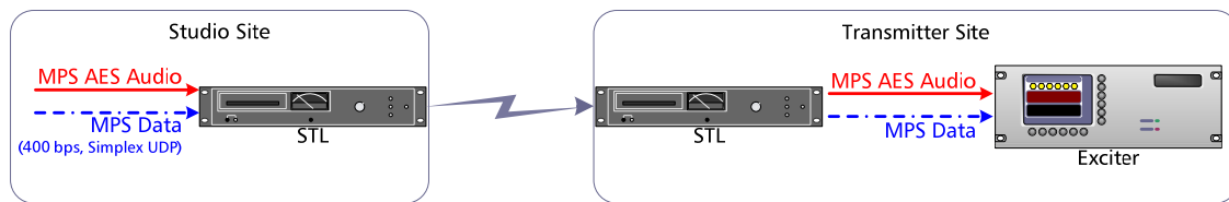
- Fig. 1: Basic HD STL Configuration, No Multicast -
