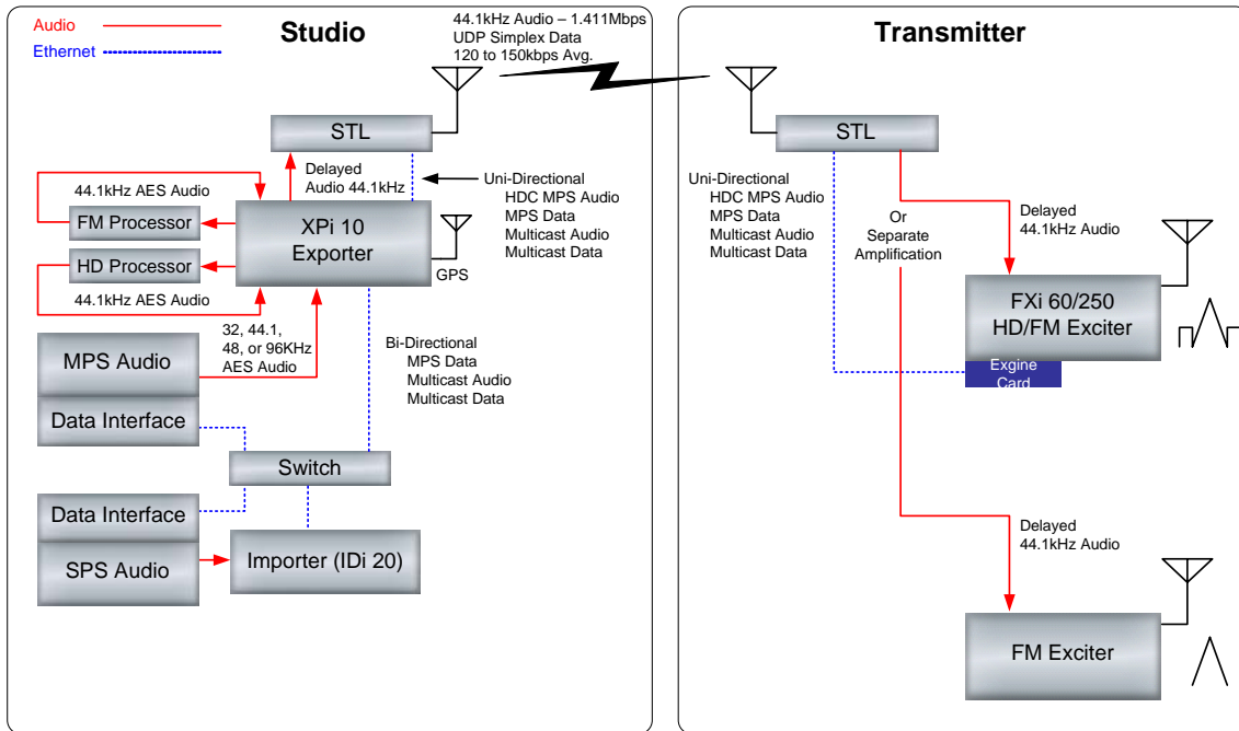
– Fig. 6: Multicast Architecture, HD Generation at Studio Site –
